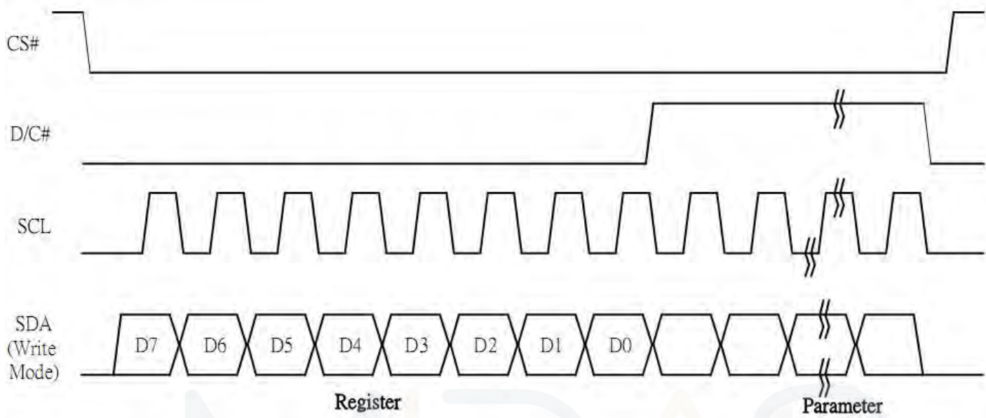
Figure 7-2 : Write procedure in 4-wire SPI mode
