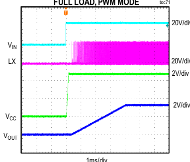
MAXM15067 STARTUP THROUGH V_{IN}
