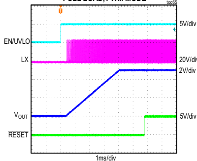
MAXM15066 STARTUP THROUGH ENABLE
