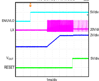
MAXM15066 STARTUP THROUGH ENABLE (2.5V PREBIAS)
