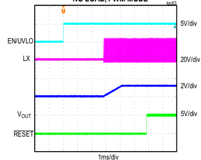
MAXM15065 STARTUP THROUGH ENABLE (2V PREBIAS)
