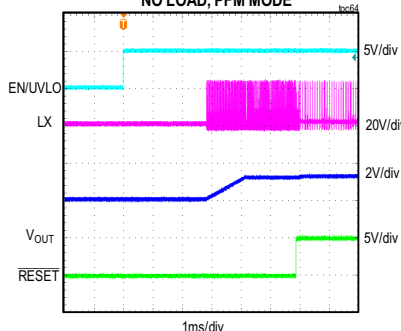
MAXM15065 STARTUP THROUGH ENABLE (2V PREBIAS)
