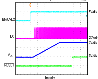
MAXM15067 STARTUP THROUGH ENABLE (2V PREBIAS)
