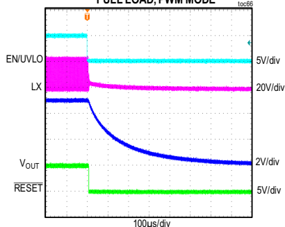
MAXM15066 SHUTDOWN THROUGH ENABLE
