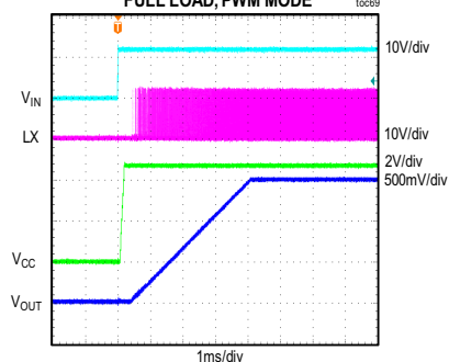
MAXM15067 STARTUP THROUGH V_{IN}
