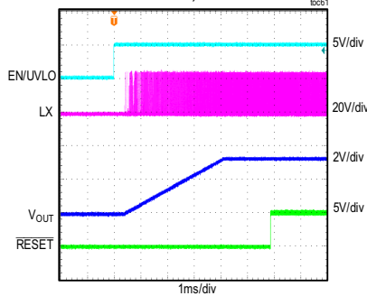
MAXM15065 STARTUP THROUGH ENABLE
