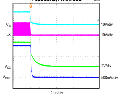
MAXM15067 SHUTDOWN THROUGH V_{IN}
