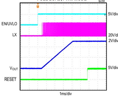
MAXM15067 STARTUP THROUGH ENABLE
