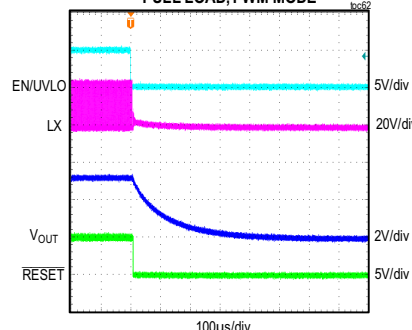
MAXM15065 SHUTDOWN THROUGH ENABLE
