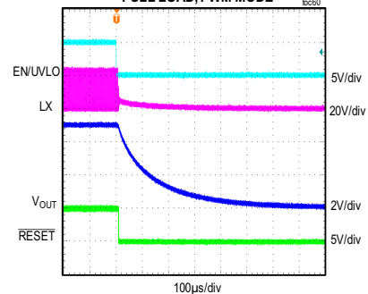
MAXM15067 SHUTDOWN THROUGH ENABLE
