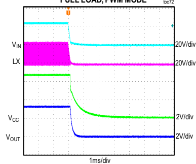
MAXM15067 SHUTDOWN THROUGH V_{IN}
