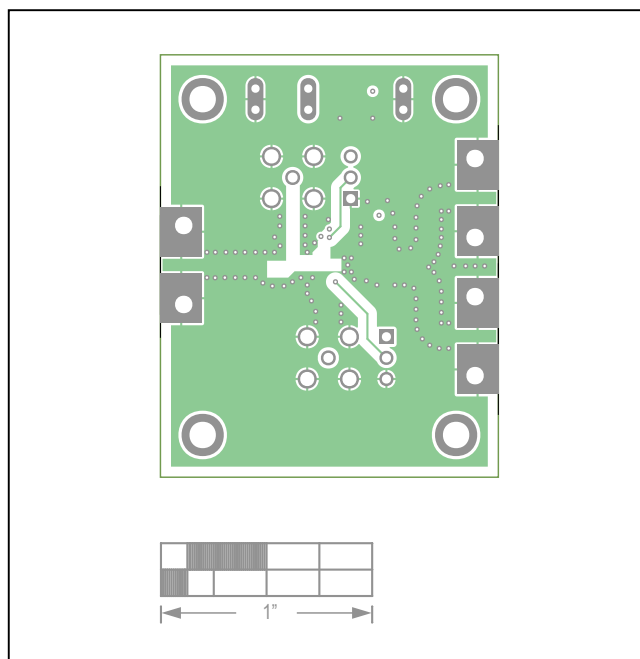
MAX40661 EV Kit—GND 3
