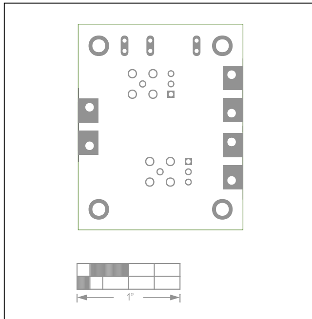
MAX40661 EV Kit—Bottom Silkscreen
