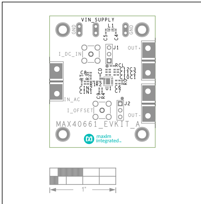
MAX40661 EV Kit—Top Silkscreen
