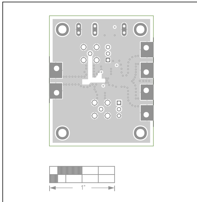
MAX40661 EV Kit—GND 2
