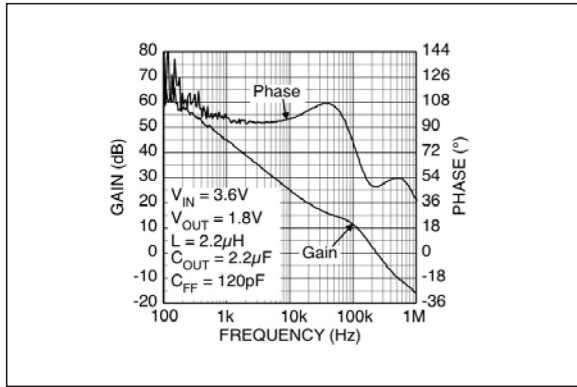
FIGURE 2-1: Bode Plot.
