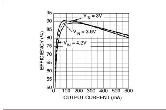
FIGURE 2-4: 1.5 V_{OUT} Efficiency.
