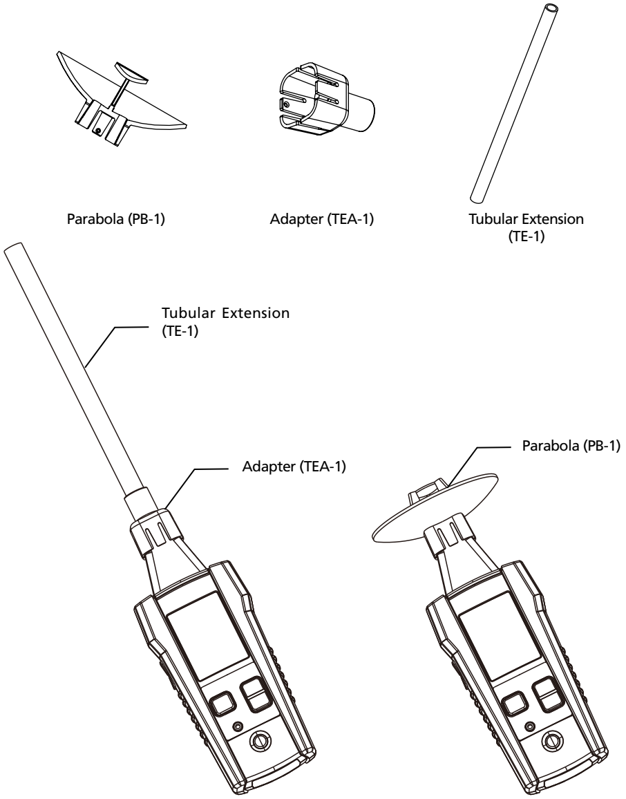
Figure 3.4: ULD-400 Accessories
