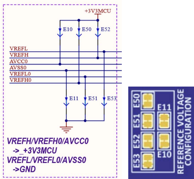
Figure 31. Analog and Reference Voltages
