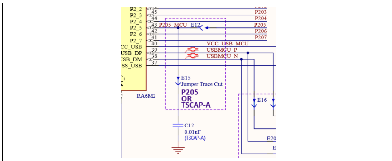
Figure 35. P205 Circuit
