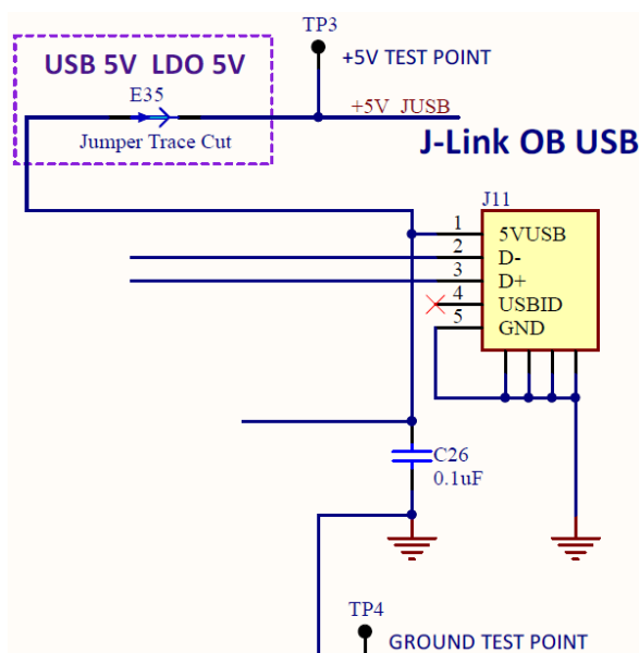
Figure 9. 5 V Power Input Circuit
