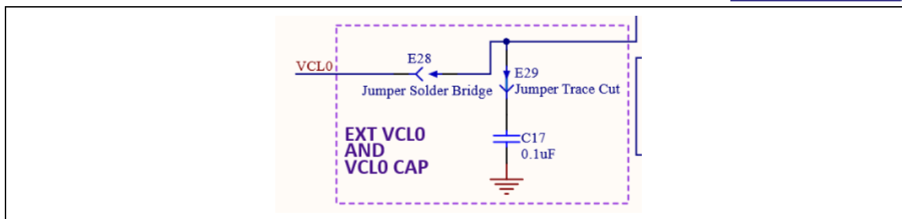
Figure 33. VCC_USB Circuit
