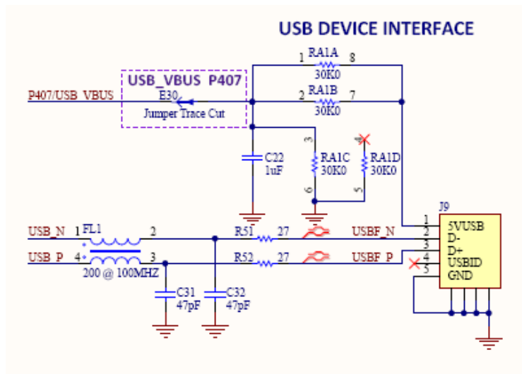
Figure 15. USB Device Interface Circuit
