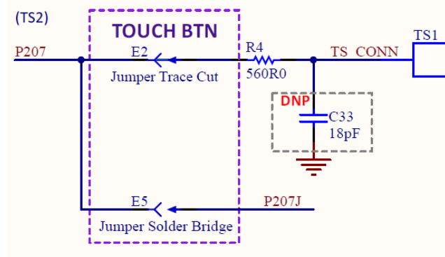
Figure 21. Capacitive Touch Button Circuit
