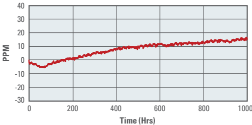
ISL21090 Long Term Drift Data (1000 Hrs)
