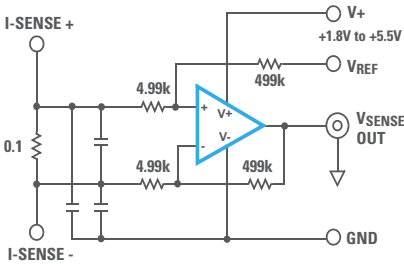
Bi-Directional Current Sense Amplifier
