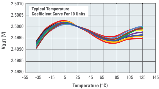
ISL21090 Typical Temperature Coefficient
