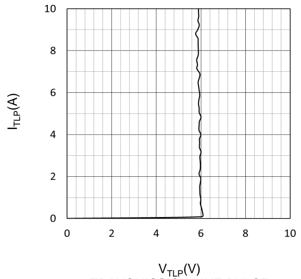
TRANSMISSION LINE PULSE
