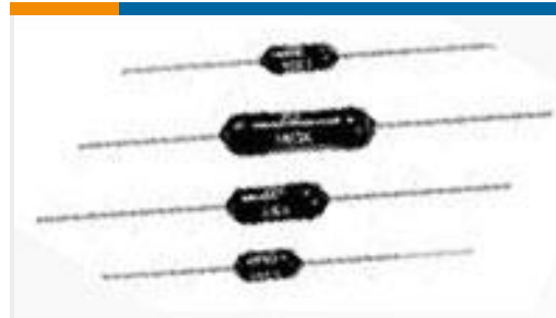
TE Model / Part #5-1879621-7 H4P 2K2 1% 50PPM
