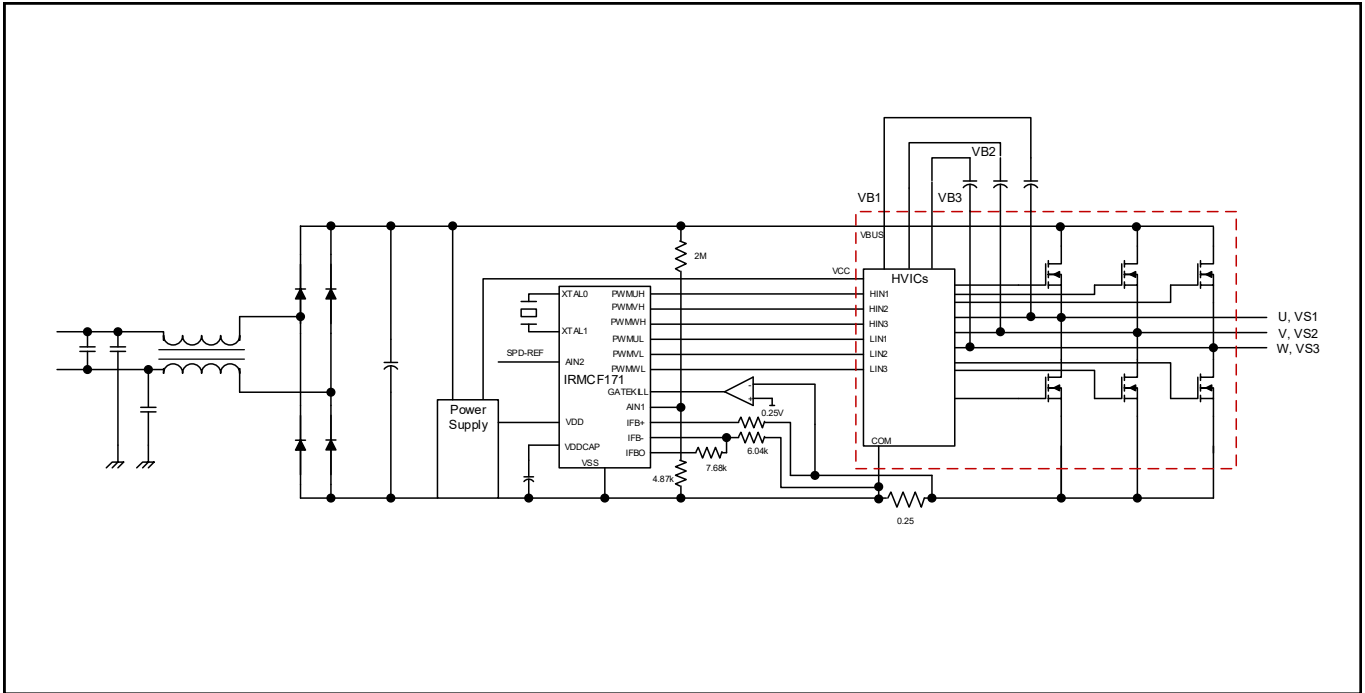
Figure 10 Application Schematic
