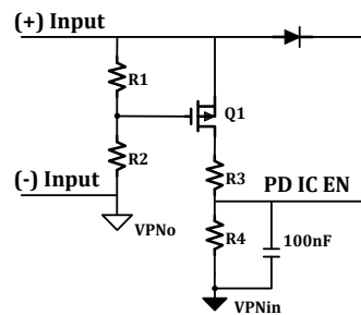
Figure 8: External Power Input resistors dividers
