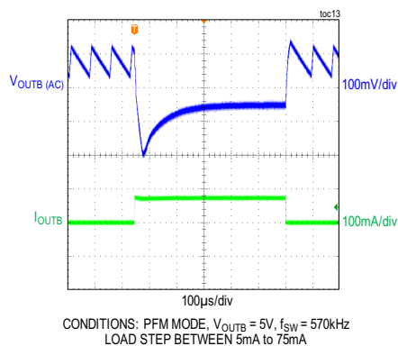
MAXM17720, MAXM17724 LOAD TRANSIENT RESPONSE
