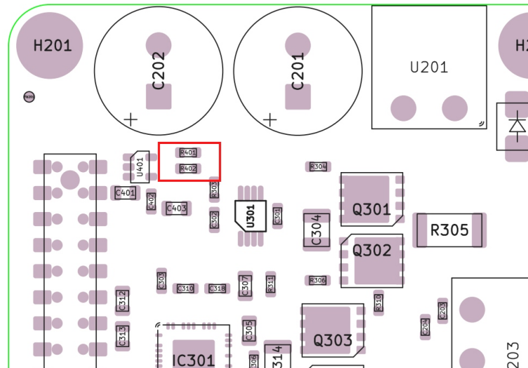
Figure 4: Solder jumper on TMC6200-EVAL
