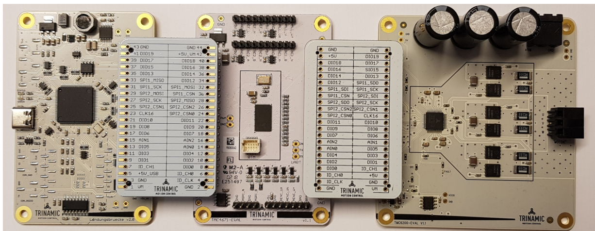
Figure 1: TMC6100-EVAL -Kit view
