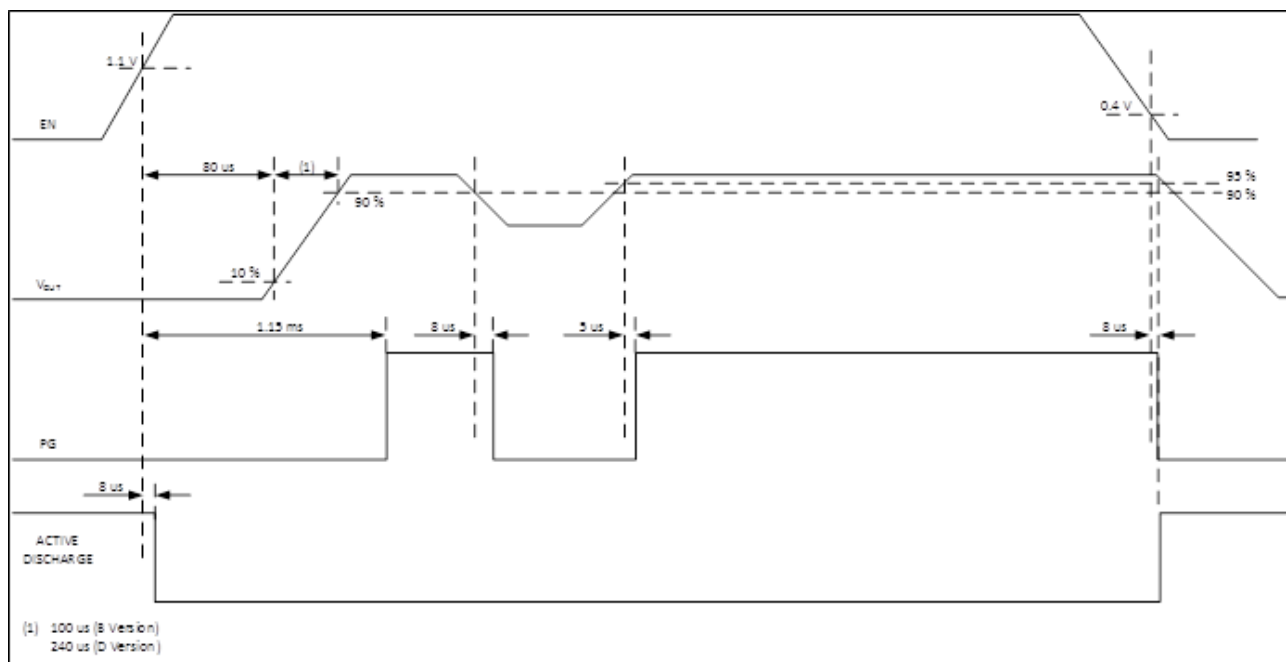
Figure 19. Power Good and Active Discharge Timing Diagram
