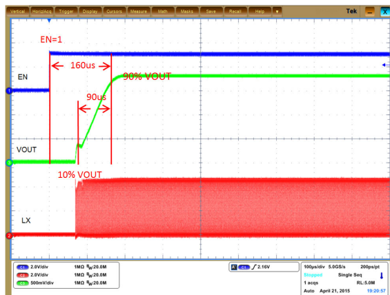
Figure 17. Soft-start Time for NCV6323B ( V_{IN} = 4.2\text{ V} , V_{OUT} = 1.8\text{ V} , I_{OUT} = 0\text{ A} , L = 1\text{ }\mu\text{H} , C_{OUT} = 10\text{ }\mu\text{F} )
