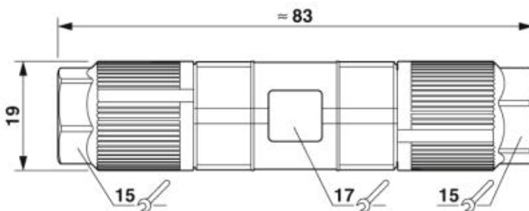
Functional drawing
