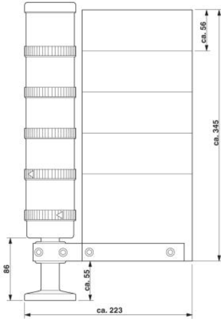
Dimensional drawing
