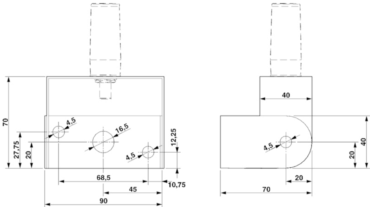
Dimensional drawing
