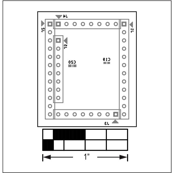
MAX20353 EV Kit—Bottom Silkscreen
