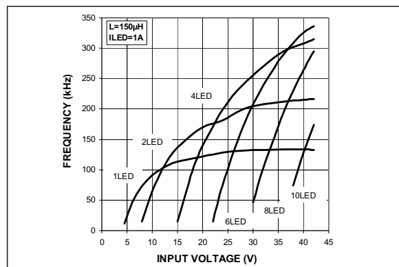
FIGURE 2-5: Frequency vs. Input Voltage ( L = 150 \mu H , I_{LED} = 1A ).
