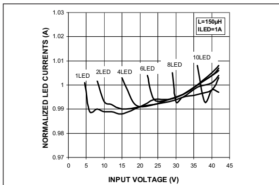
FIGURE 2-3: Normalized LED Currents vs. Input Voltage ( L = 150 \mu H , I_{LED} = 1A ).
