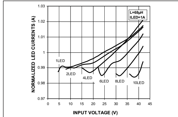
FIGURE 2-4: Normalized LED Currents vs. Input Voltage ( L = 68 \mu H , I_{LED} = 1A ).
