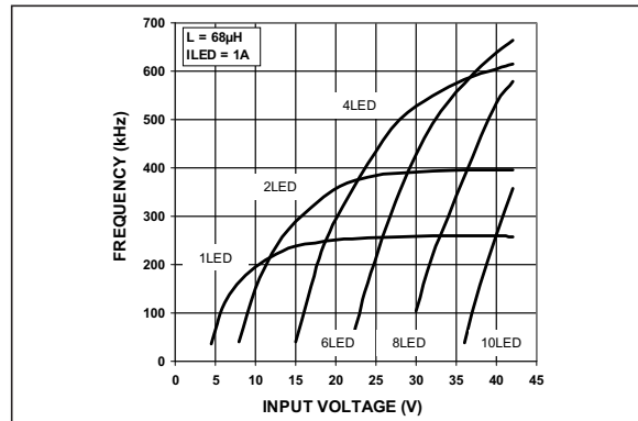
FIGURE 2-6: Frequency vs. Input Voltage ( L = 68 \mu H , I_{LED} = 1A ).
