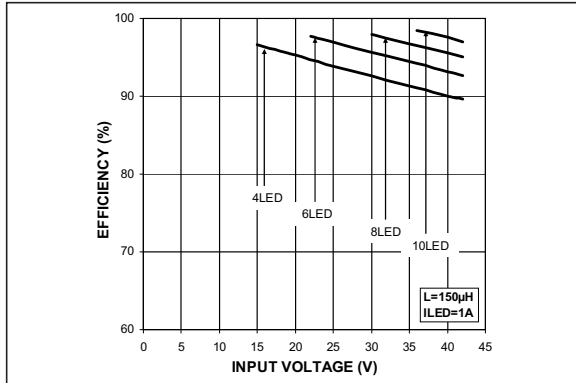
FIGURE 2-1: Efficiency vs. Input Voltage ( L = 150 \mu H , I_{LED} = 1A ).
