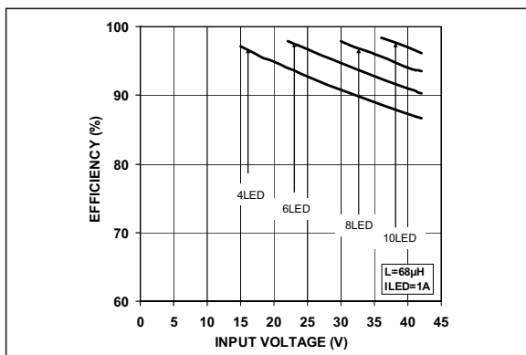
FIGURE 2-2: Efficiency vs. Input Voltage ( L = 68 \mu H , I_{LED} = 1A ).
