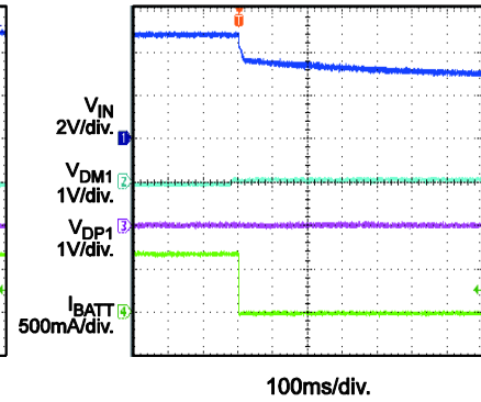
USB Removal, No Load Connection
