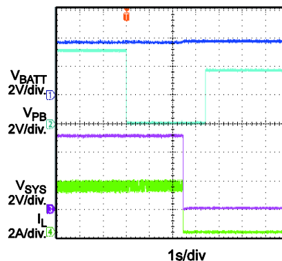
Power Off by PB, Boost Mode
