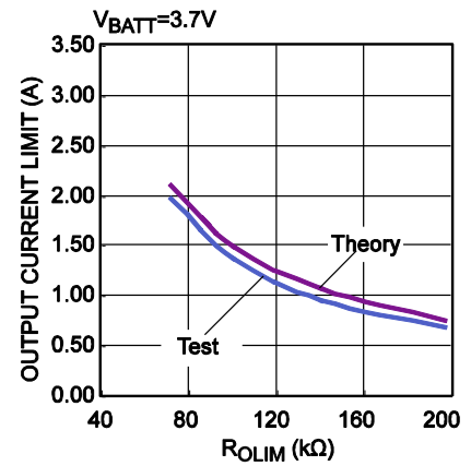
Programmable Output Current Limit, Boost Mode
