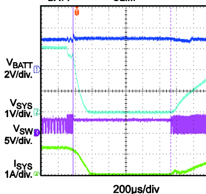
Auto Restart after SYS OCP, Boost Mode
