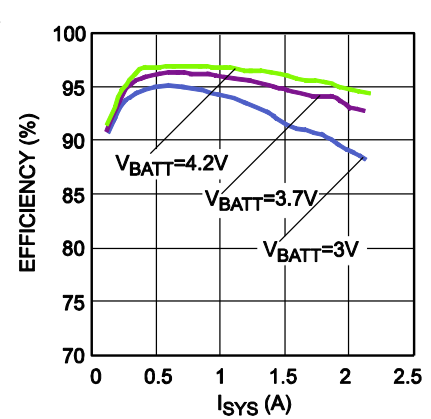
Boost Efficiency R_{OLIM}=0
