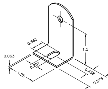
Brackets Dimensions
