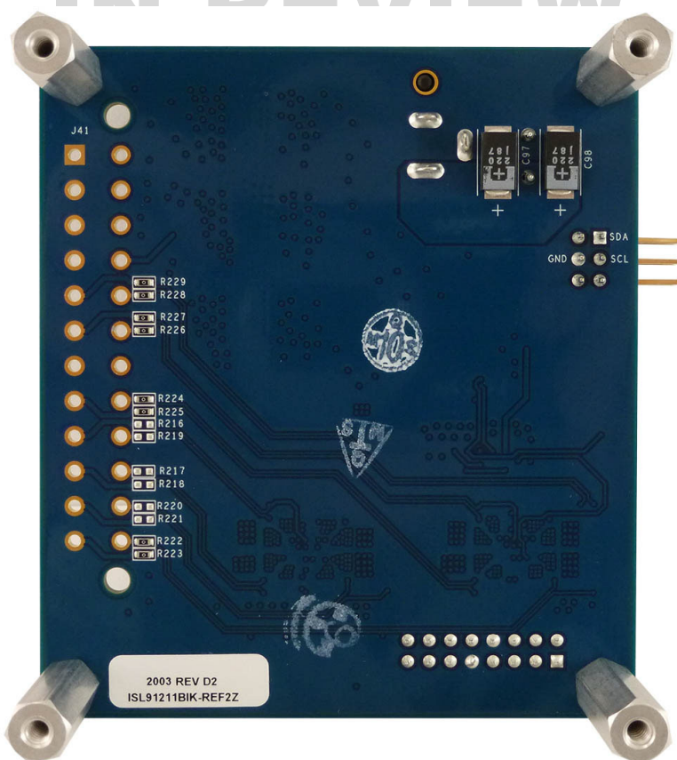
Figure 42. ISL91211BIK-REF2Z Bottom
