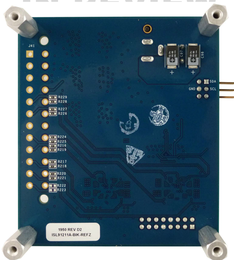
Figure 40. ISL91211A-BIK-REFZ Bottom
