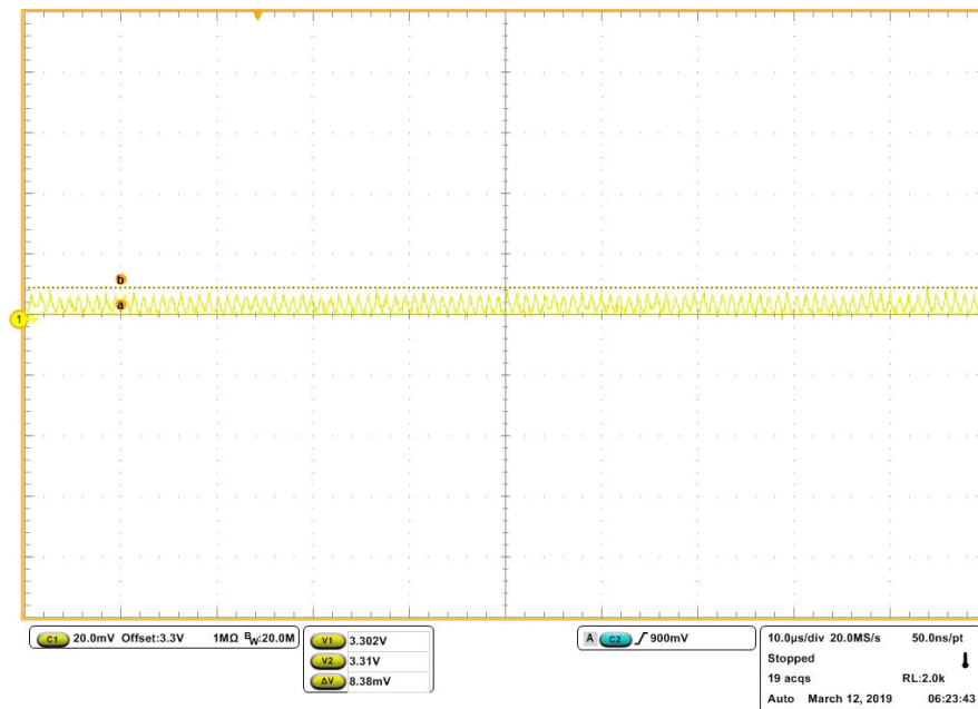
Figure 34. VCCO 3.3V Output Ripple at 3A, <8.3mV_{P-P}
