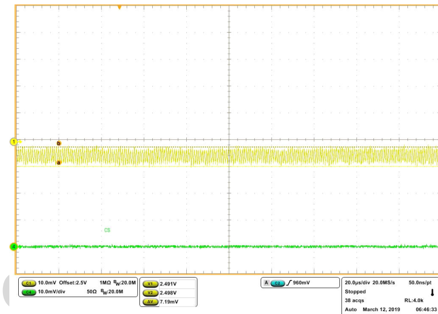
Figure 30. VCCO 2.5V Output Ripple at No Load, <7.19mV p-p
