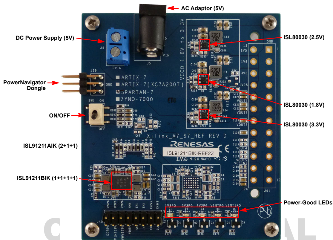
Figure 41. ISL91211BIK-REF2Z Top
