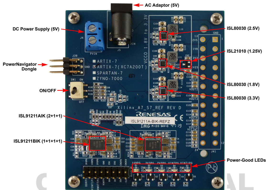
Figure 39. ISL91211A-BIK-REFZ Top
