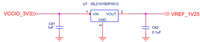
ISL21010DFH312 for 1.25V reference to FPGA ADC
