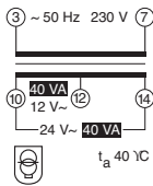
TS40/12-24 C
