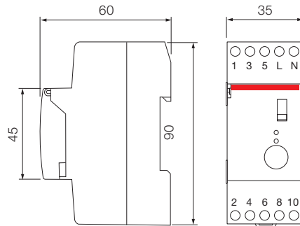
TW2/10K
