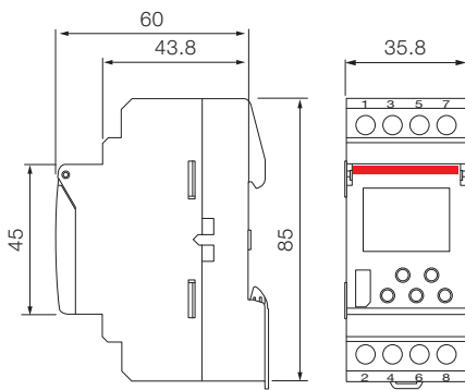
TWA-1
