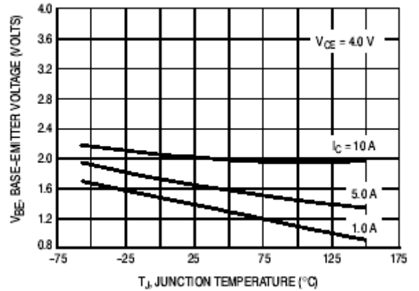
Base-Emitter Voltage
