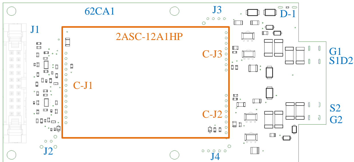
Figure 2 62CA1 Interconnects on Adapter Board
