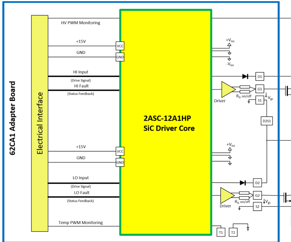
Figure 1 62CA1 Adapter Board Basic Topology
