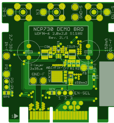
Figure 79. WDFN-6 2x2 Demo Board (2 layer, rev. 1) – PCB Top Layer
