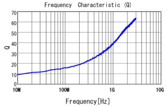
■ LQG15HS1N0S02 Q
