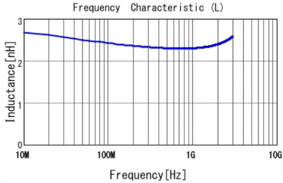
■ LQG15HS2N4S02 L
