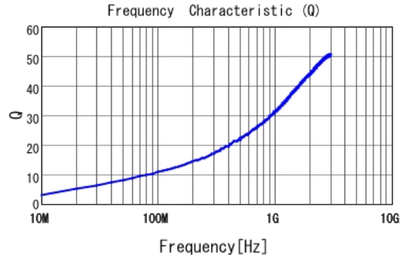
■ LQG15HS2N4S02 Q
