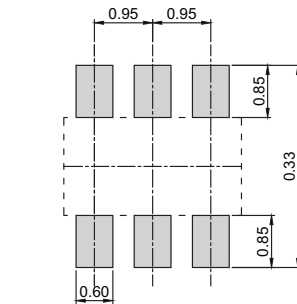
Recommended soldering pad layout (unit :mm)
