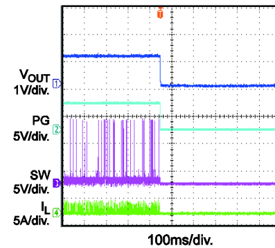
Thermal Shutdown V_{IN}=19V , I_{OUT}=0.1A
