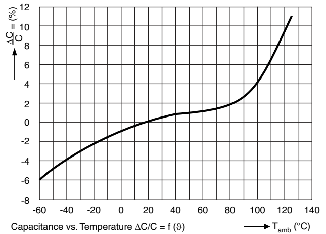
Capacitance vs. Temperature \Delta C/C = f (°) \rightarrow T_{amb} (°C) Capacitance as a function of temperature (typical curve)
