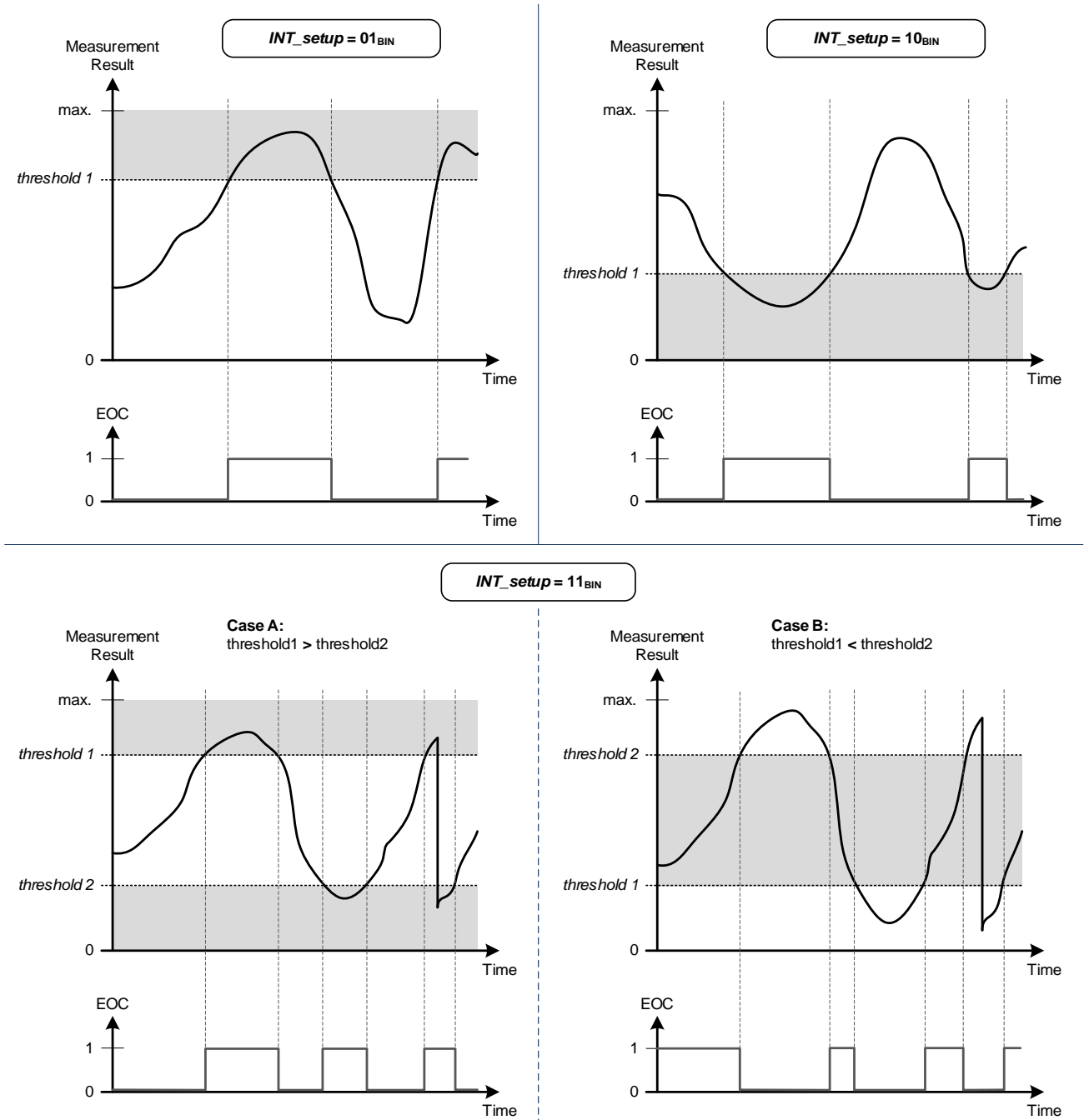
Figure 21. EOC and Interrupt Thresholds
