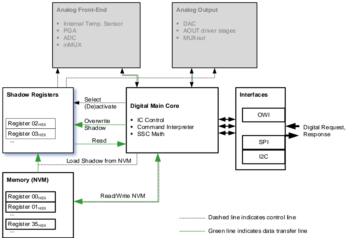
Figure 22. Digital IC Section Architecture
