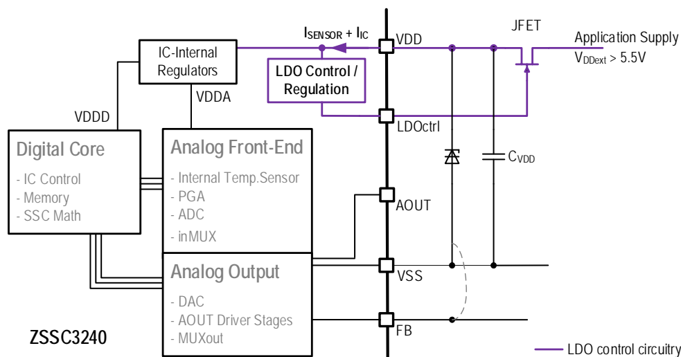
Figure 23. LDOctrl Application Topology
