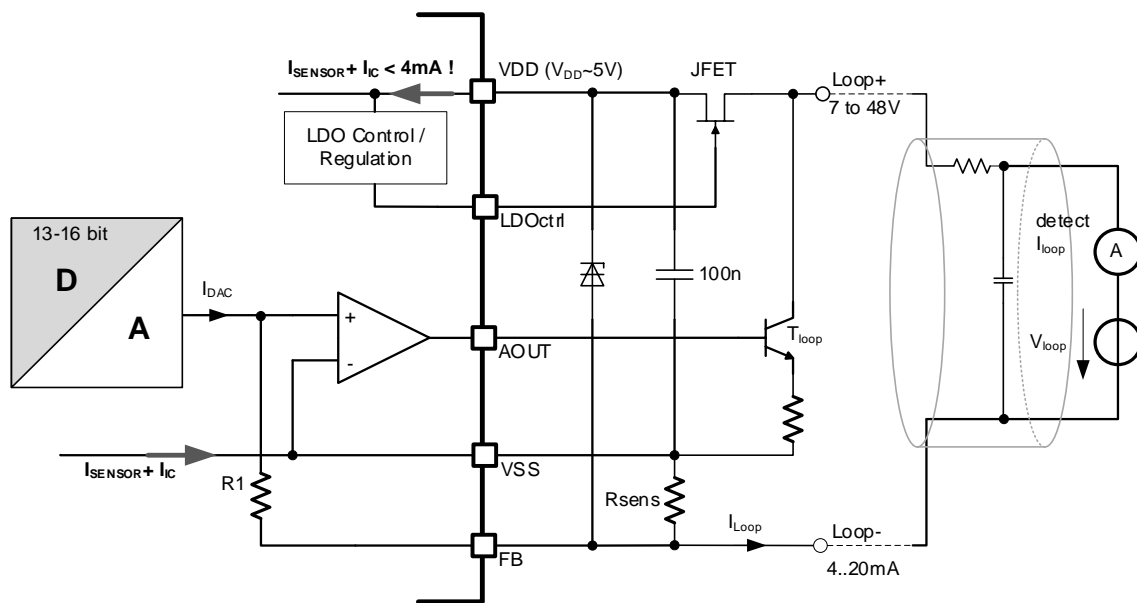
Figure 20. Current Loop Configuration
