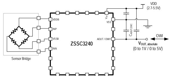
Analog Sensor with Absolute Voltage Out
