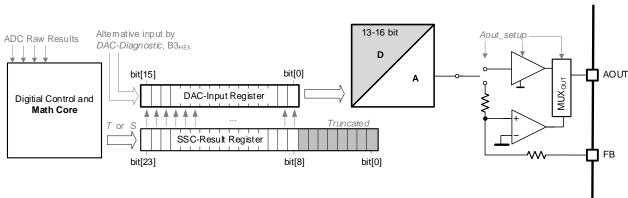
Figure 19. DAC and Analog Output Topology
