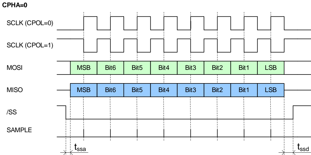
Figure 5. SPI Configuration CPHA=0
