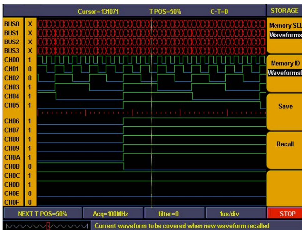
Fig.5-74: Waveform saving
