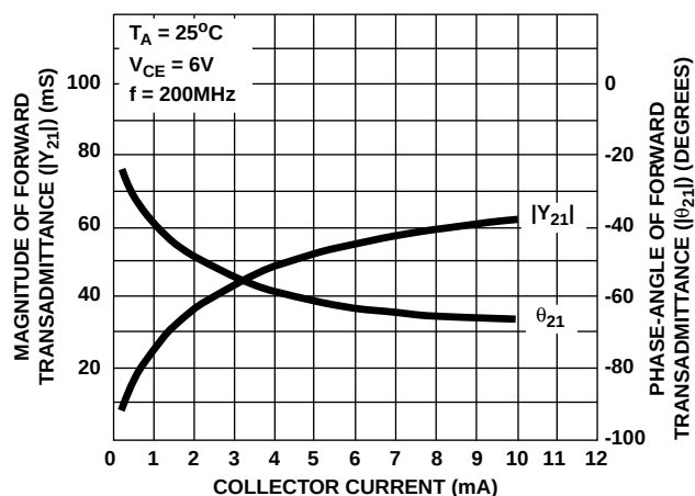
FIGURE 16. FORWARD TRANSMITTANCE ( Y_{21} ) vs COLLECTOR CURRENT
