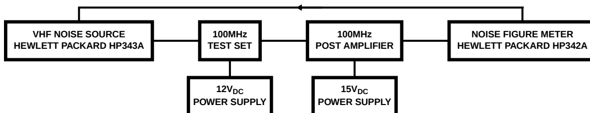
FIGURE 3B. NOISE FIGURE SET-UP
