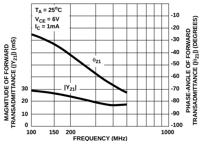
FIGURE 17. FORWARD TRANSMITTANCE ( Y_{21} ) vs FREQUENCY
