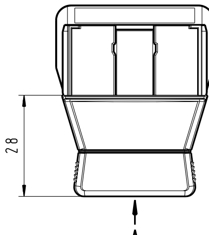
ROW-Stecker/plug 1809281
