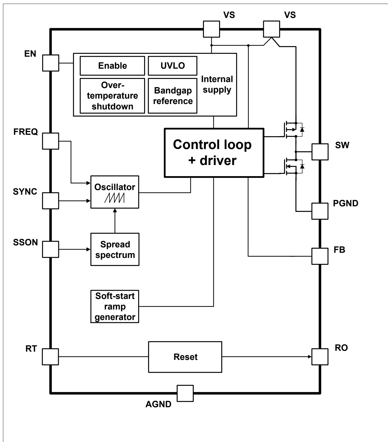
Figure 1 Block diagram
