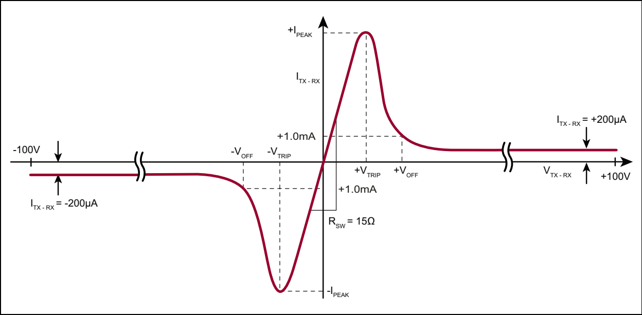
Typical I-V Characteristics
