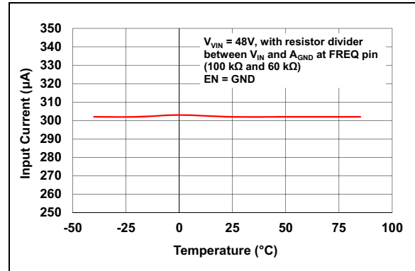
FIGURE 2-4: Input Shutdown Current vs. Temperature.
