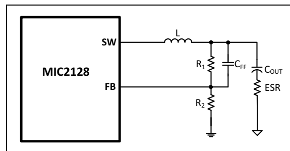
FIGURE 5-6: Inadequate Ripple at FB.
