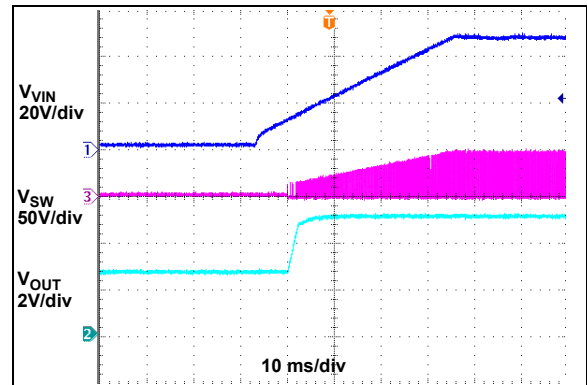
FIGURE 2-28: V_{IN} Turn-On with Pre-biased Output.
