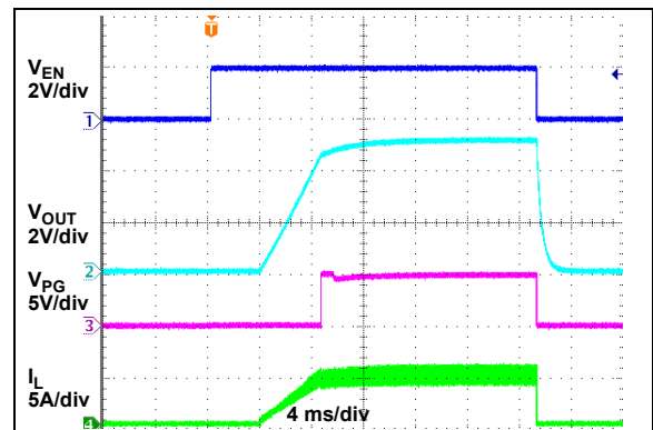
FIGURE 2-29: EN Turn-On/Turn-Off.
