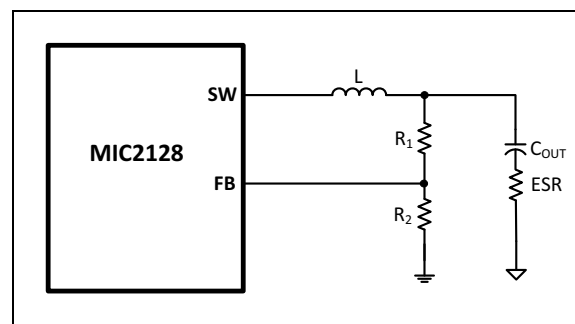
FIGURE 5-5: Enough Ripple at FB.
