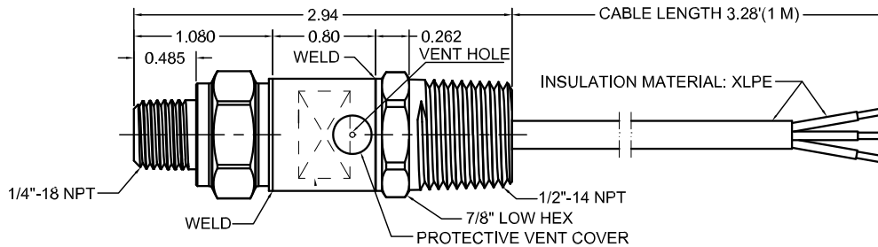
Figure 1. Model BWA-PRESSURE-SENSOR-50
