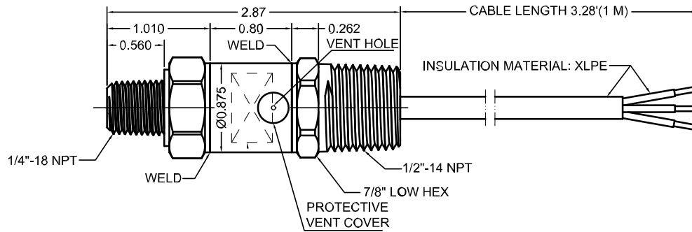
Figure 1. Model BWA-PRESSURE-SENSOR-50
