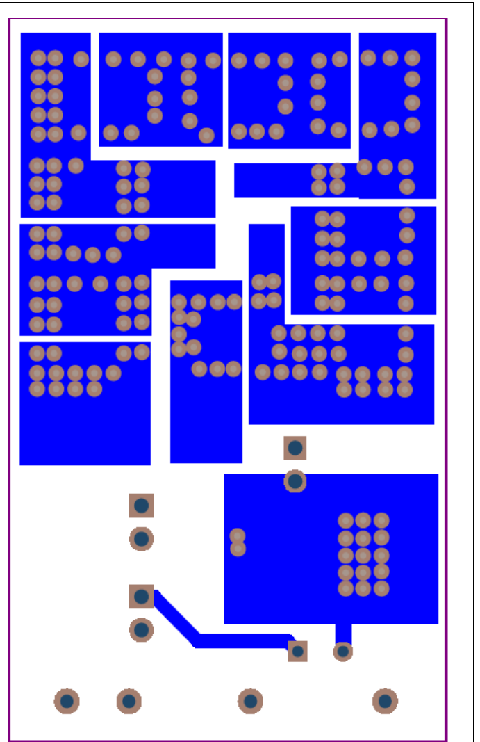
Figure 5 Layout bottom
