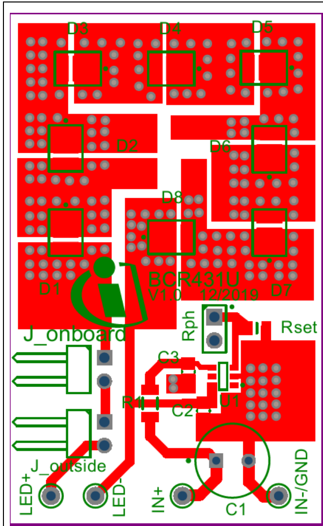
Figure 4 Layout top
