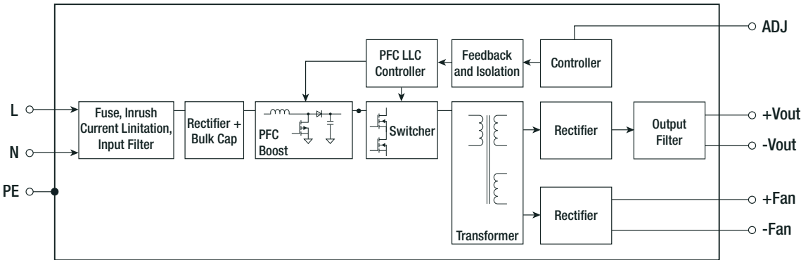
Block Diagram
