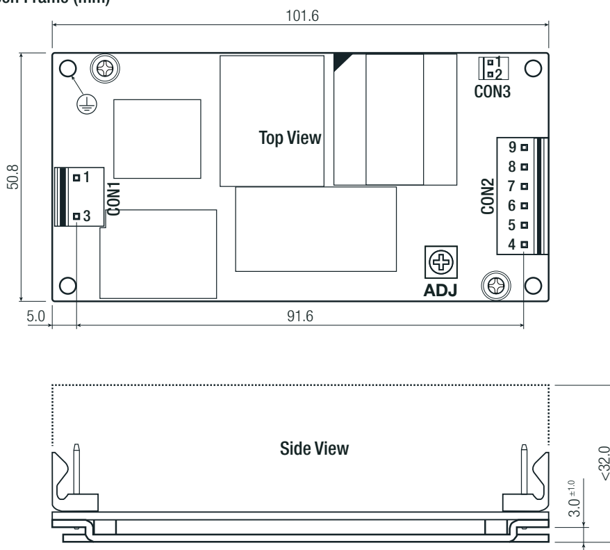
Dimension Drawing Open Frame (mm)
