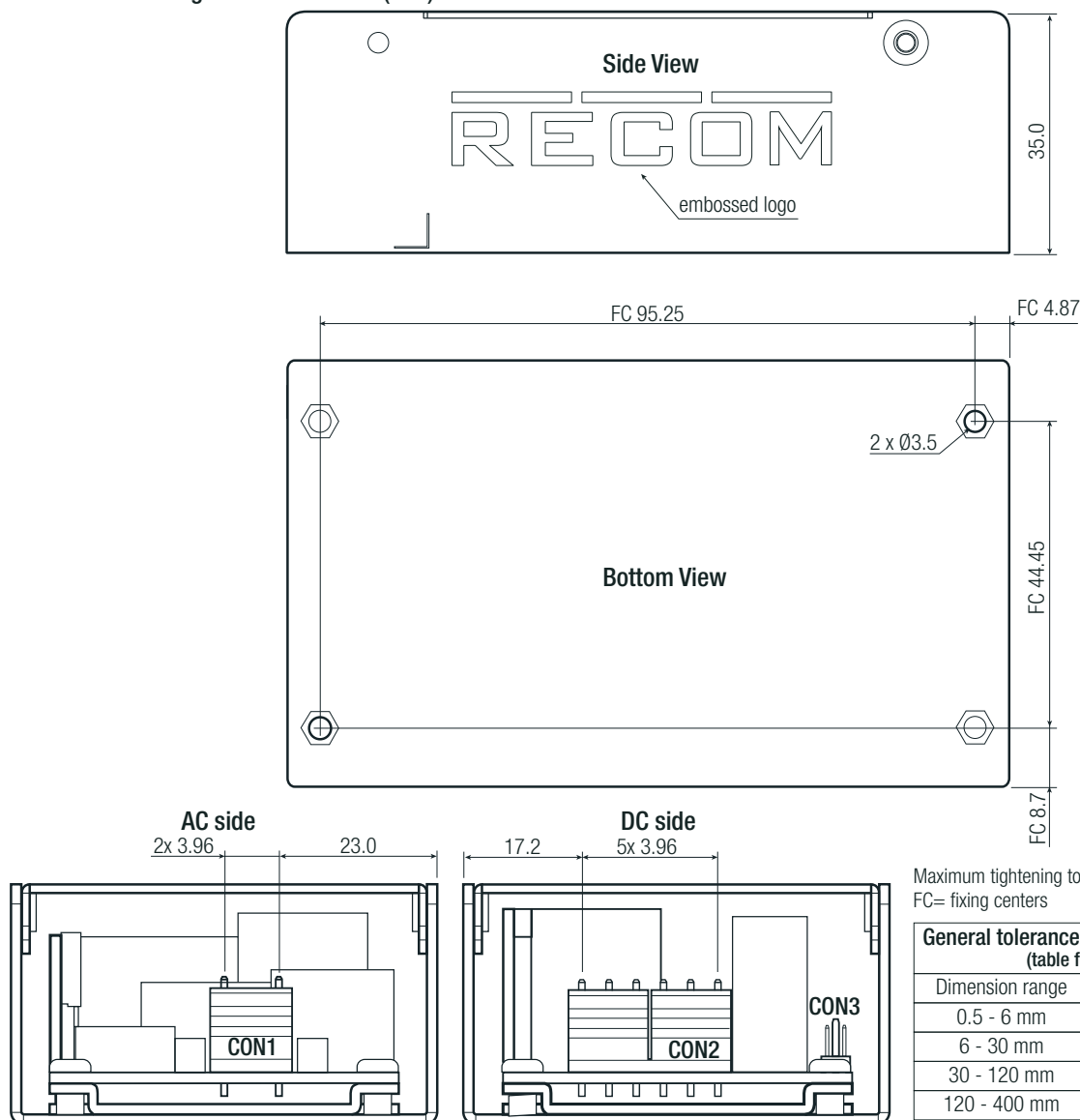
Dimension Drawing Enclosed Version (mm)
