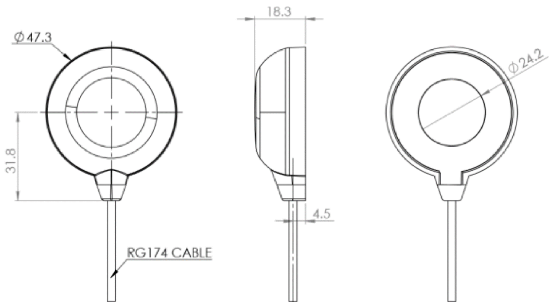
Figure 17: GNSS antenna dimensions (mm)
