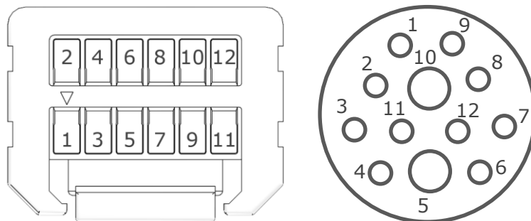
Figure 14: Numbering 12-pin connectors; left Molex (cable entry view), right ODU (solder cup view).
