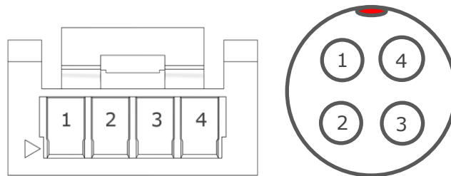
Figure 16: Numbering 4-pin connectors; left Molex (cable entry view), right ODU (solder cup view).
