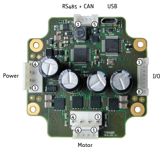
Figure 2: TMCM-1260 connectors
