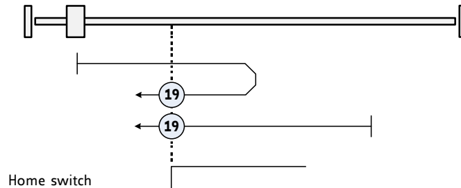
Figure 21: Homing Method 19
