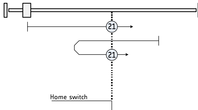
Figure 22: Homing Method 21
