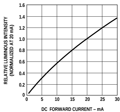
Figure 5. Relative intensity vs. DC forward current.
