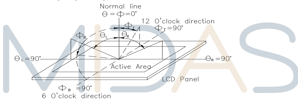
Fig.11.1. Definition of viewing angle
