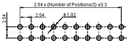
PCB Layout
