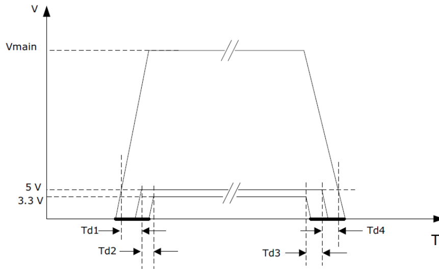
Figure 4-2. Power Sequencing
