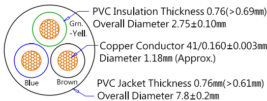
SJT 18AWGx3C (Wire Cross-Section)
